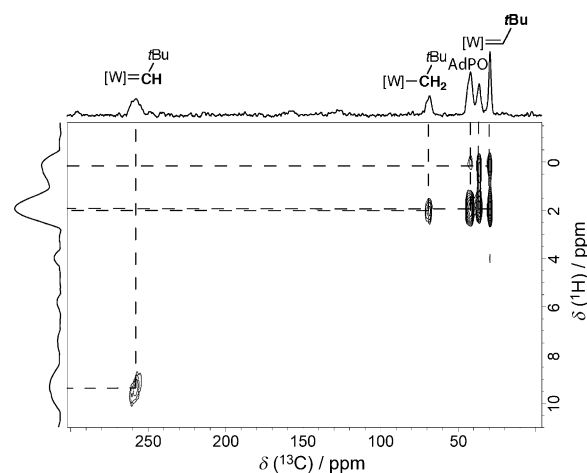
Figure 1. Two-dimensional 1 H– 13 C HETCOR spectrum of 2b recorded with a CP contact time of 600 μs. Other experimental details are given in the Supporting Information. The one-dimensional 13 C CPMAS spectrum is shown above the two-dimensional plots together with the assignment of the resonances.
