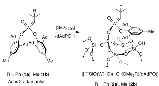
Scheme 2. Selective formation of 2a by grafting 1a on silica partially dehydroxylated at 700 °C.
